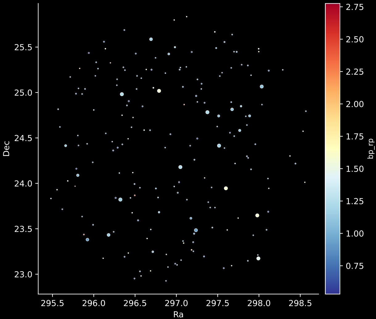
APOGEE DR17 Field: [357+85_MGA] Stars: 191
