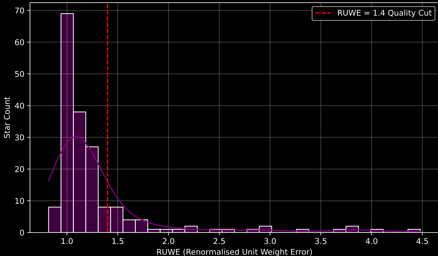
GAPOGEE DR17 Field [357+85_MGA] RUWE Distribution (n= 182)
