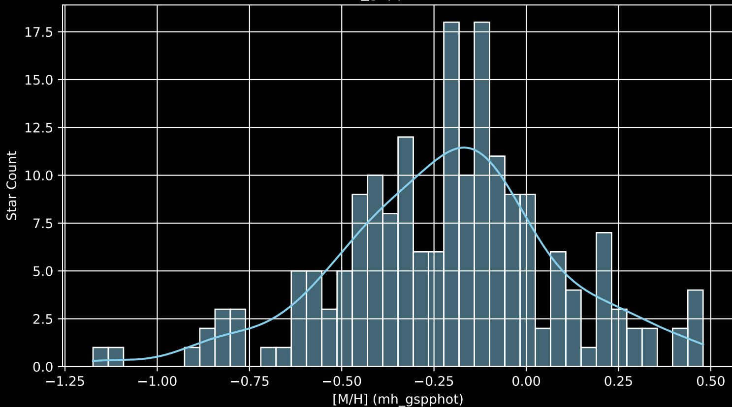
APOGEE DR17 Field: [357+85_MGA [M/H] (mh_gspphot) (n= 190)
