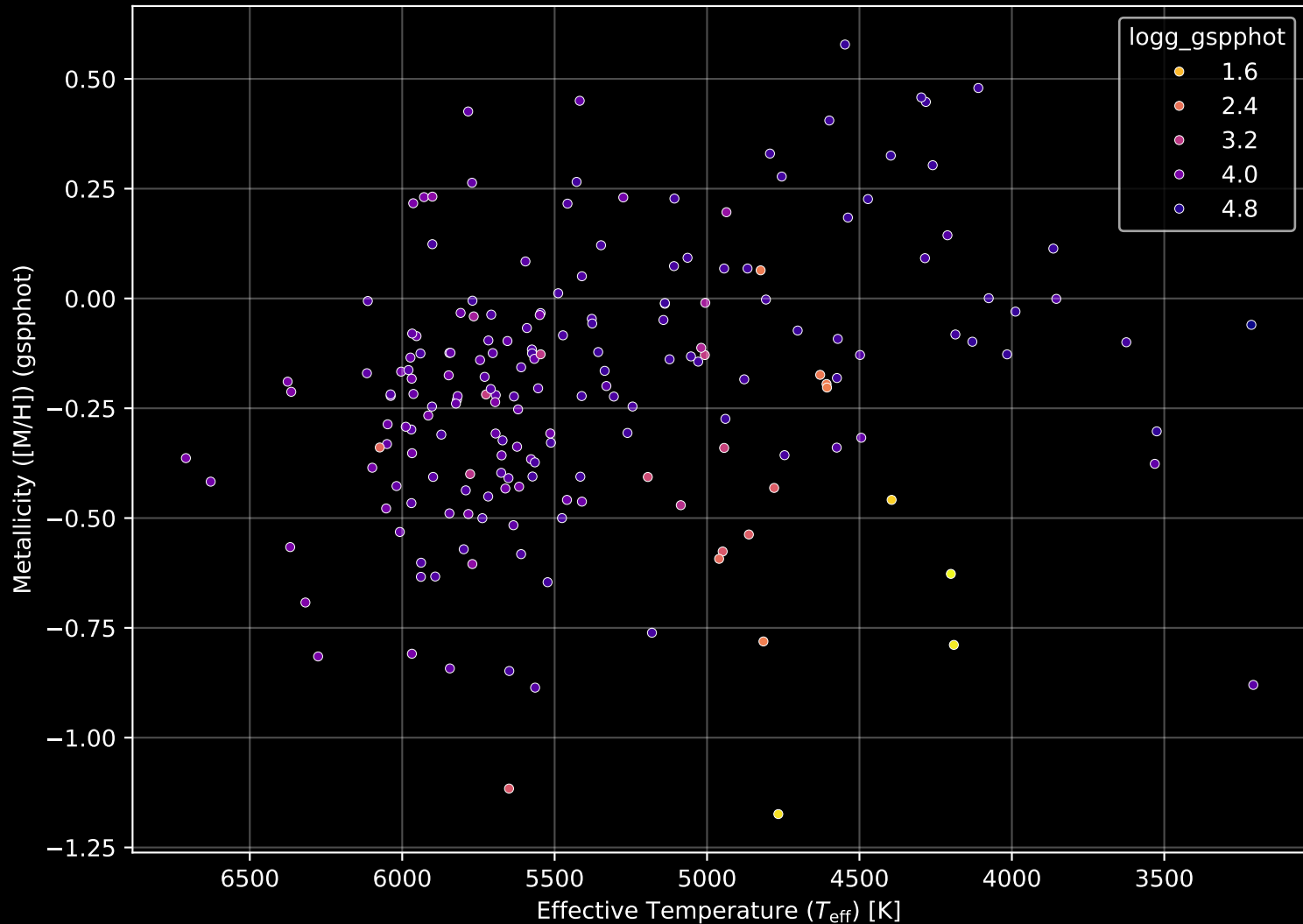
APOGEE DR17 Field: [357+85_MGA] Stellar Population Parameters (n= 191)
