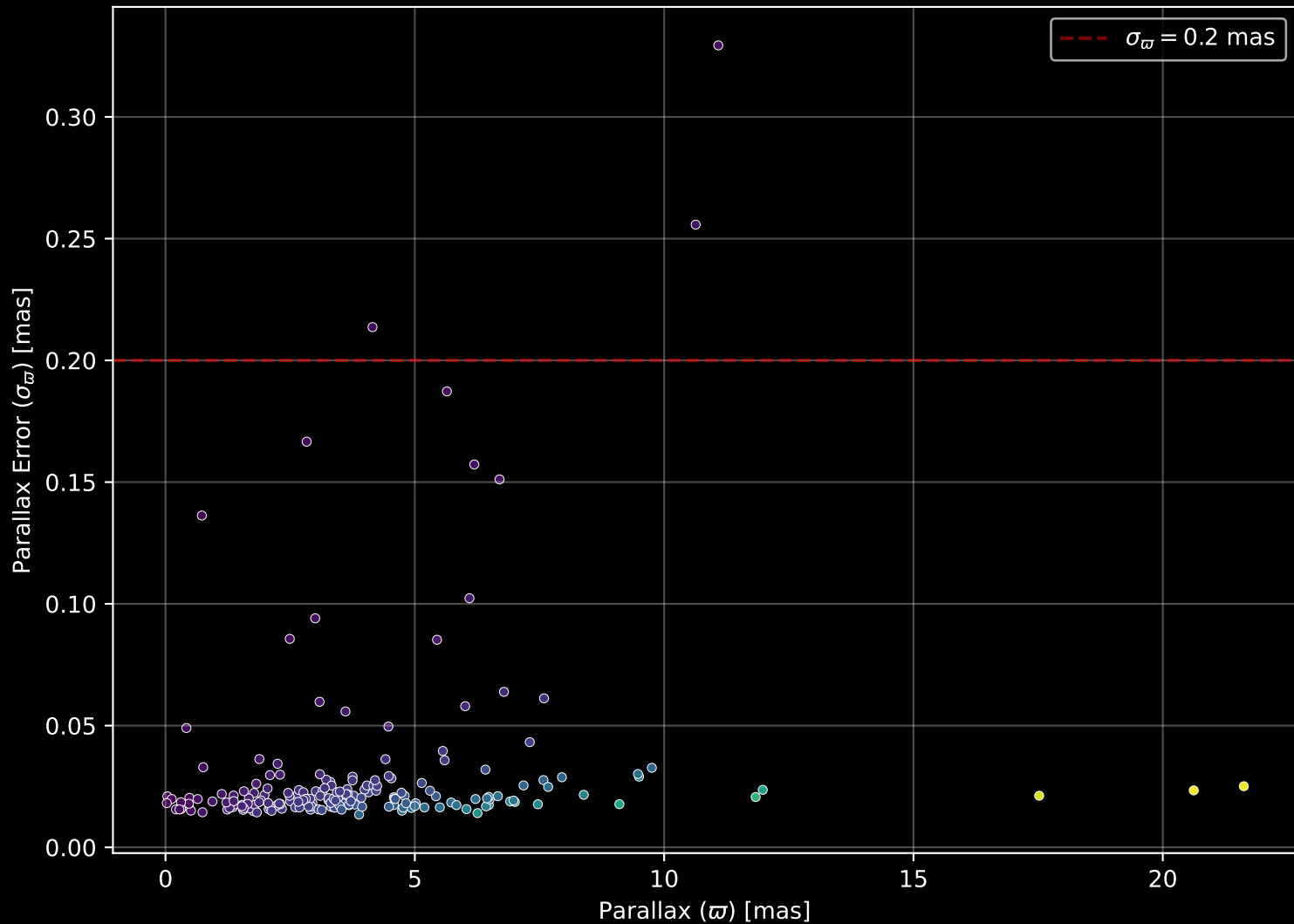
APOGEE DR17 Field: [357+85_MGA] Parallax Quality (n= 191)
