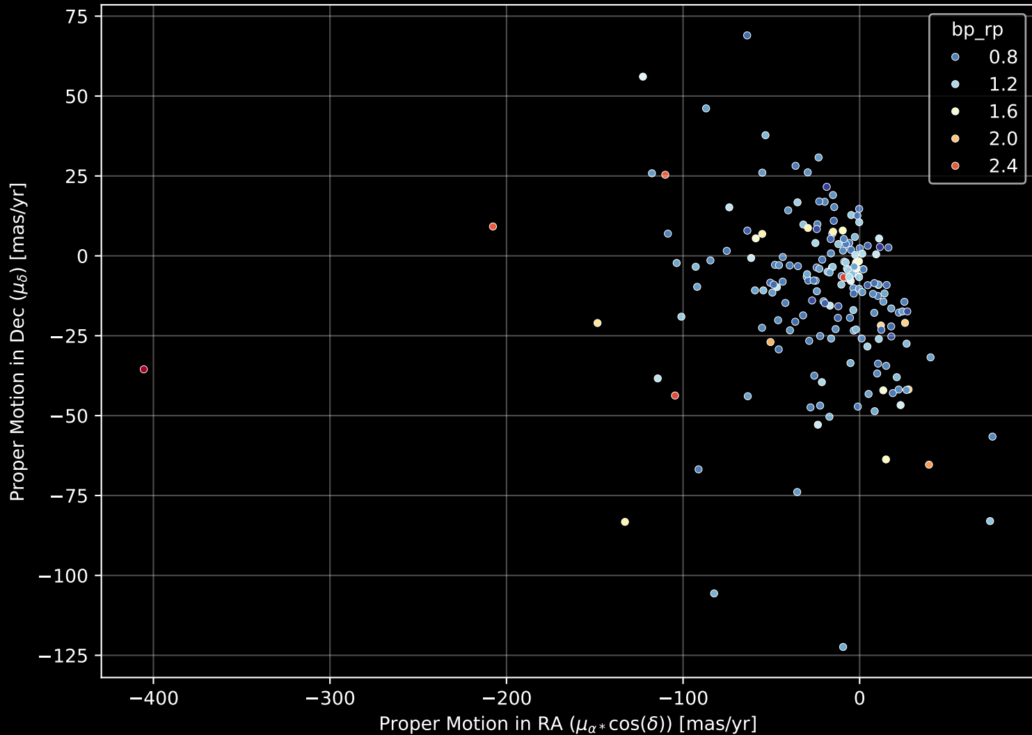
APOGEE DR17 Field: [357+85_MGA] Proper Motion Diagram (n= 191)
