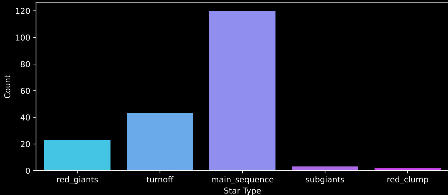
APOGEE DR17 Field: [357+85_MGA] Count plot of Star Type
